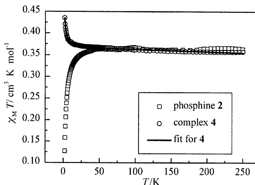
Fig. 3 Temperature dependence of \chi_M T for the phosphine 2 and the complex 4 . The solid line represents the analytical fit based on a chain model of S = 1/2 spins in ferromagnetic interaction.
