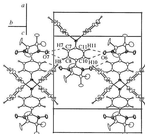
Fig. 2 View of the crystal lattice along the b direction showing the spin carriers alignment [the Mo(CO) 5 moieties along the c axis have been omitted]. Selected intermolecular distances (Å): O(6)⋯O(7) 3.892(8), O(6)⋯C(10) 3.33(2), O(6)⋯H(10) 2.66, O(6)⋯C(11) 3.40(2), O(6)⋯H(11) 2.86, O(7)⋯C(7) 3.472(19), O(7)⋯H(7) 2.821, O(7)⋯C(8) 3.44(2), O(7)⋯H(8) 2.81. Mean angle between two adjacent nitronyl nitroxide groups 0°.
